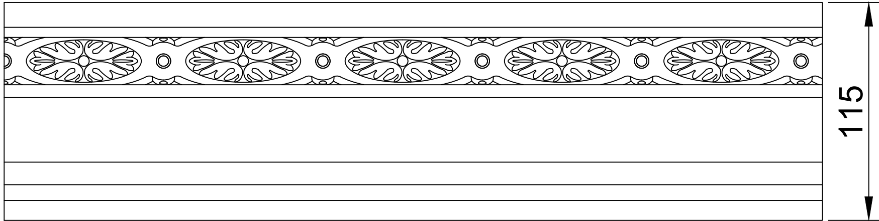
Front Scale 1:2
