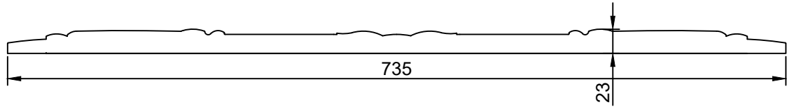
Side Scale 1:5
